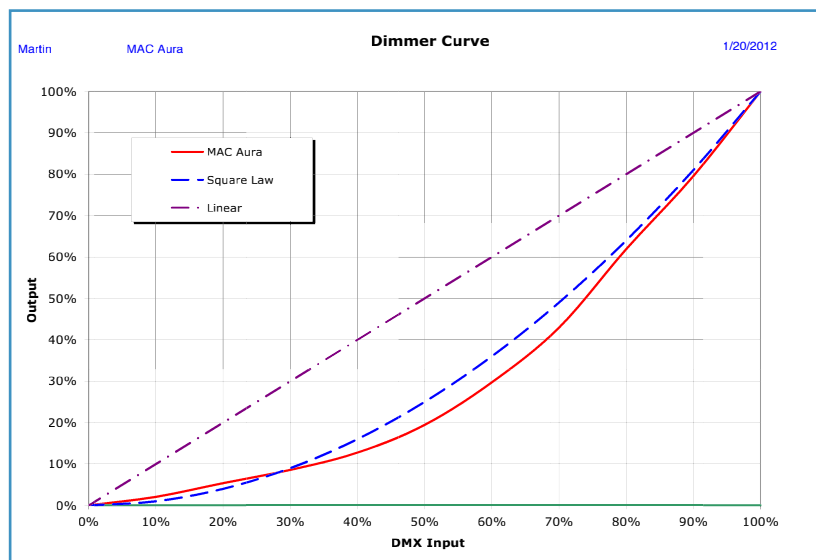
Figure 8: Dimmer curve
