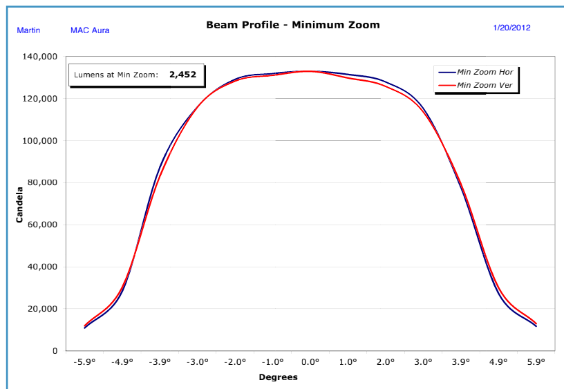
Figure 7: Minimum zoom
