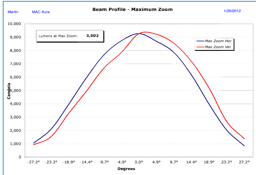
Figure 6: Maximum zoom
